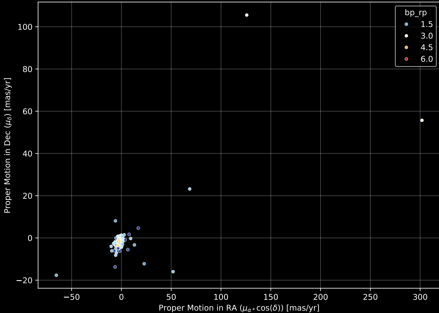
APOGEE DR17 Field: [105+00] Proper Motion Diagram (n= 157)
