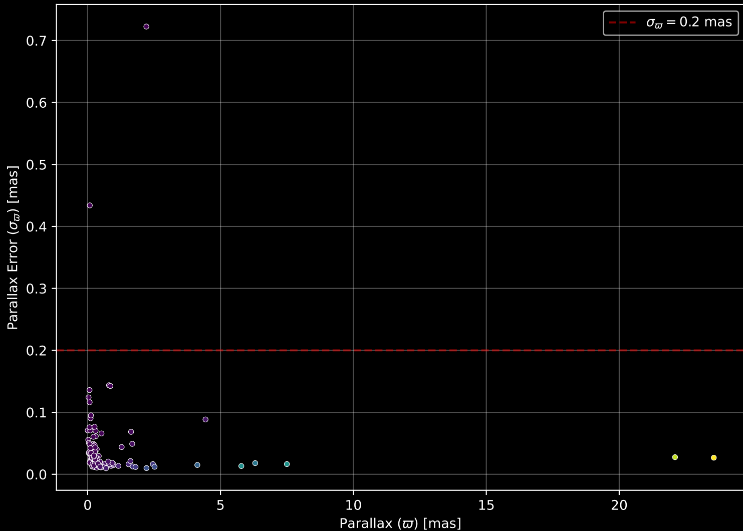
APOGEE DR17 Field: [105+00] Parallax Quality (n= 157)
