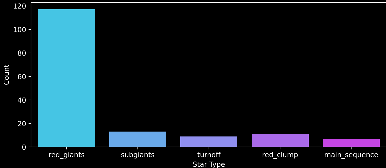
APOGEE DR17 Field: [105+00] Count plot of Star Type
