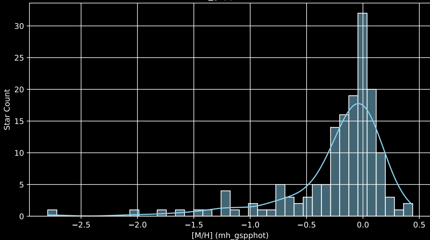
APOGEE DR17 Field: [105+00 [M/H] (mh_gspphot) (n= 155)
