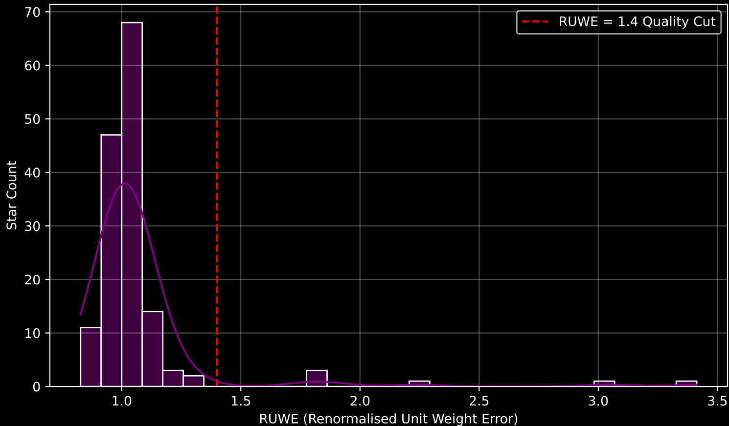
GAPOGEE DR17 Field [105+00] RUWE Distribution (n= 151)
